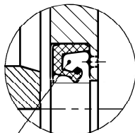
Detail II
