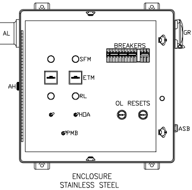
ENCLOSURE AND DEADFRONT LAYOUT (TYPICAL) (OUTER DOOR REMOVED)
