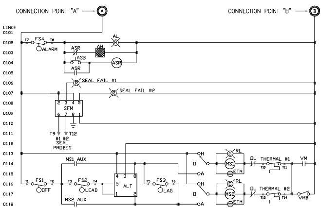
CONTINUATION OF WIRING DIAGRAMS FROM ABOVE
