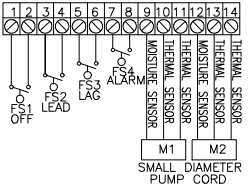
TERMINAL STRIP
