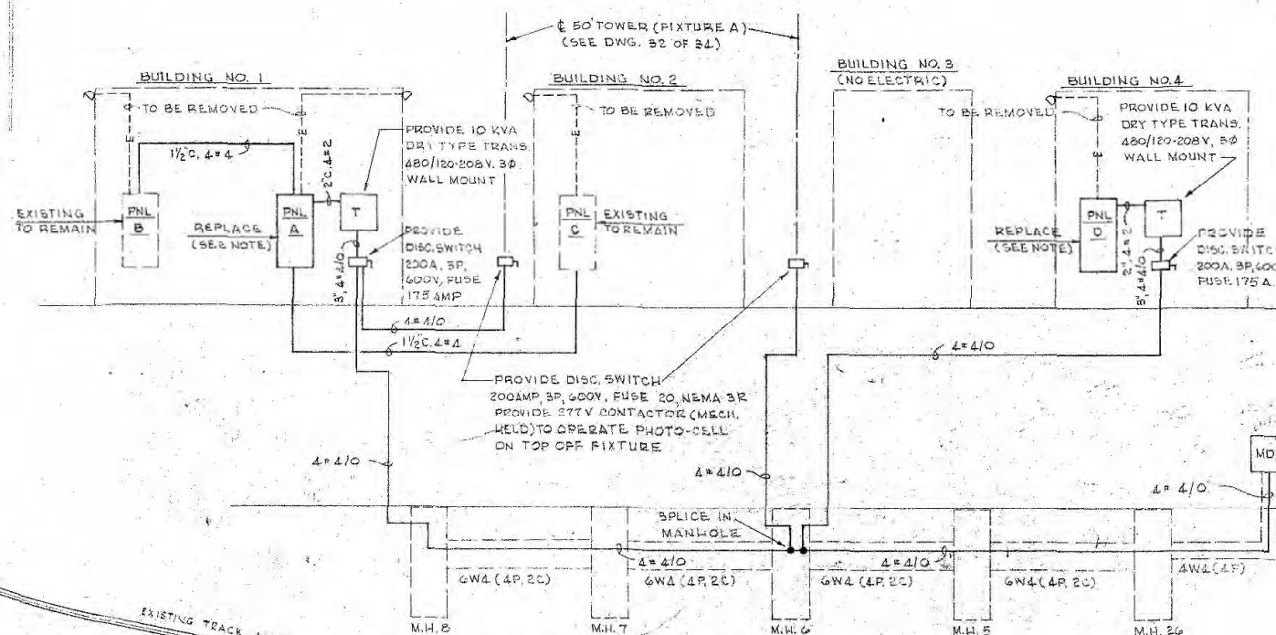
ONE-LINE WIRING DIAGRAM- CORPS OF ENGINEER'S PROPERTY
