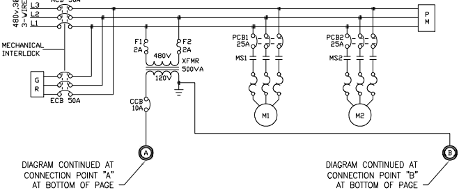
480V THREE PHASE WIRING DIAGRAM
