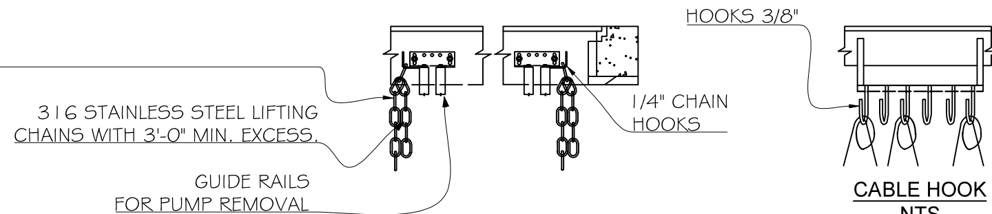
CHAIN HOOK & RAIL BRACKET NTS
