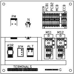
BASE PLATE LAYOUT (TYPICAL)
