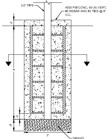
1 6 POLE EMBEDMENT DETAIL SCALE 1" = 2'
