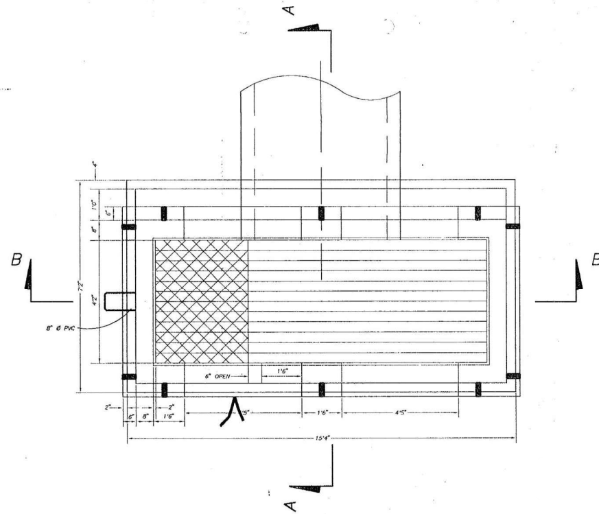
PLAN VIEW (EXISTING STRUCTURE)
