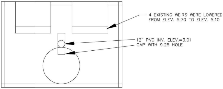
POND 8 OUTFALL STRUCTURE AS-BUILT MODIFICATION DETAIL NOT TO SCALE
