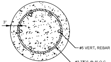
1 7 POLE EMBEDMENT TOP VIEW SCALE 1" = 2'
