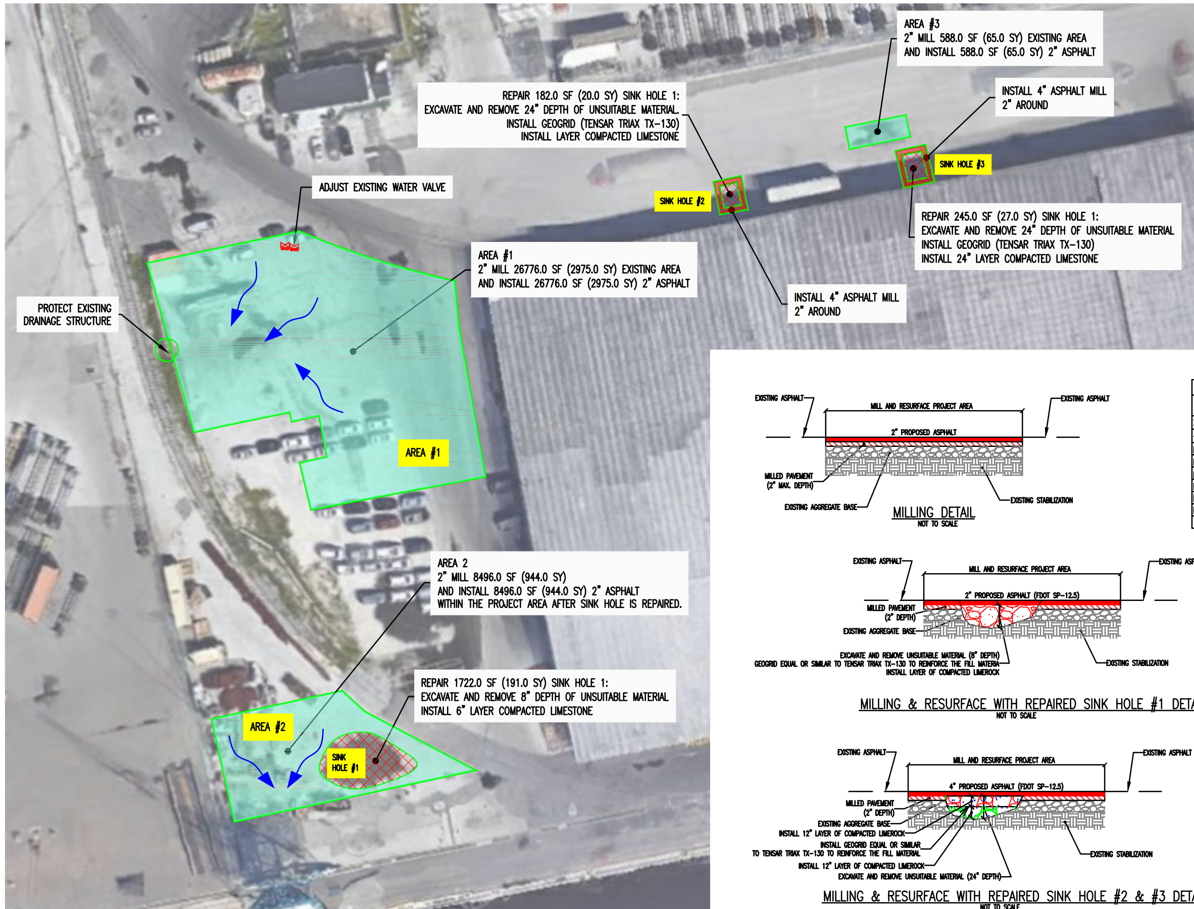
PLAN VIEW
