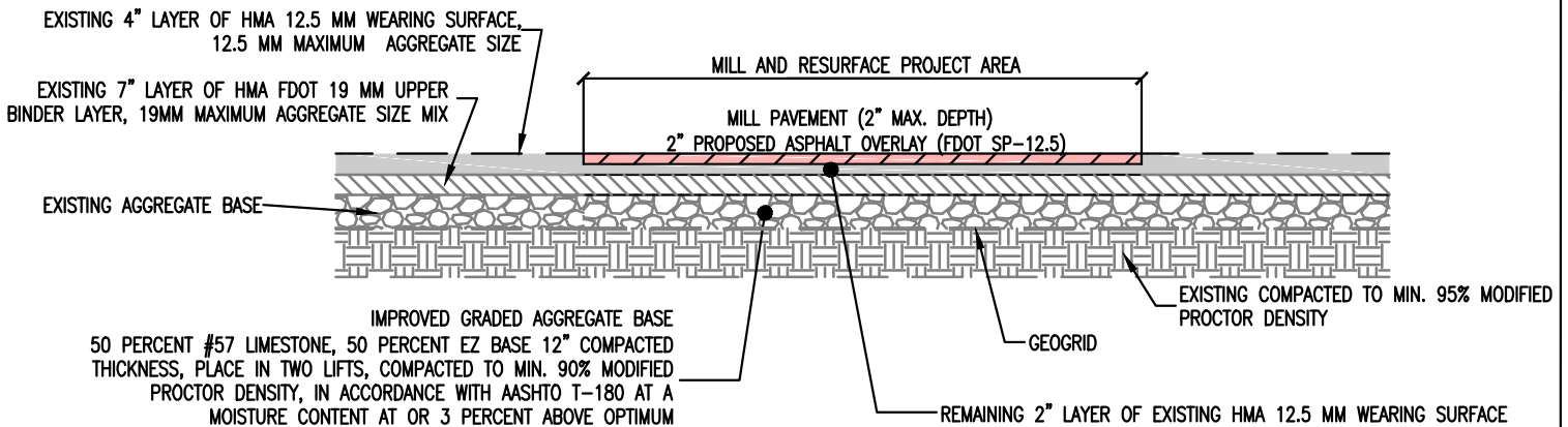
MILLING DETAIL NOT TO SCALE
