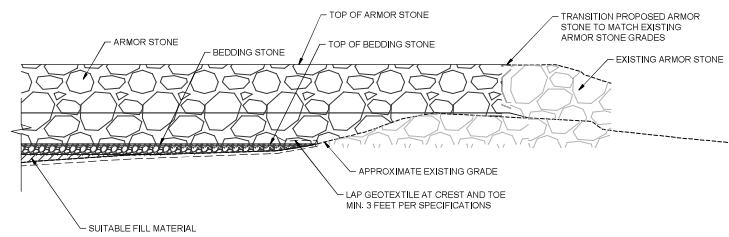
A5 ELEVATION DETAIL AT END OF REVETMENT (STA. 7+36) 22x34: 1" = 6' 11x17: 1" = 12'
