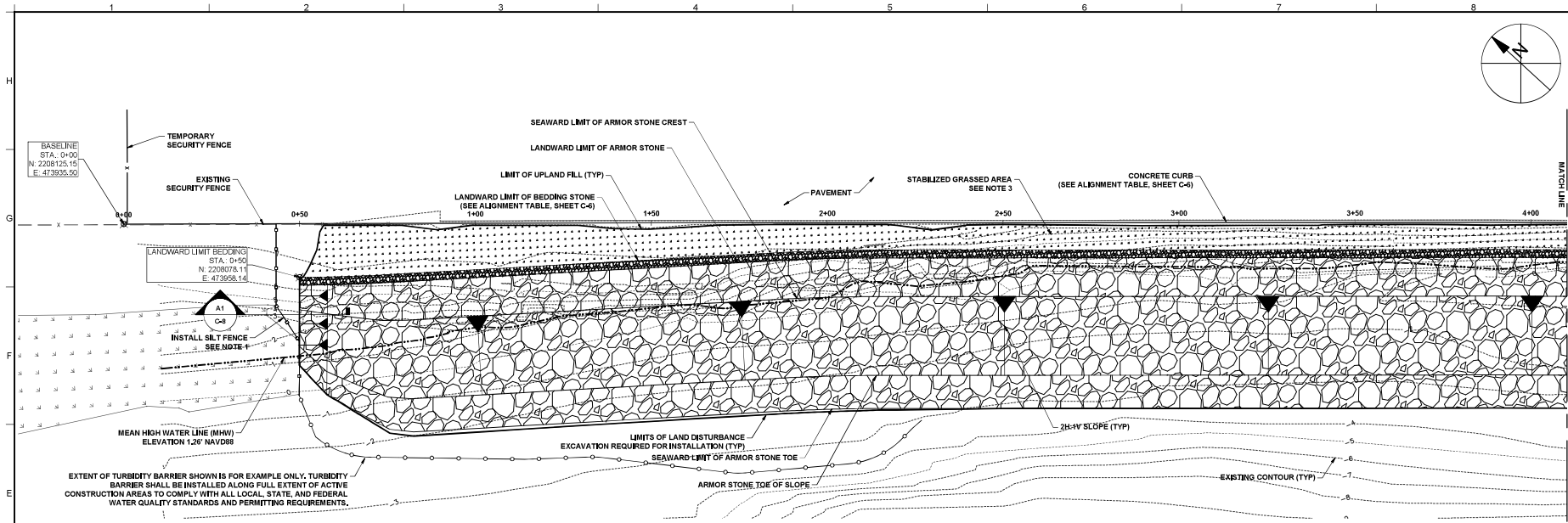
E1 REVETMENT PLAN - STA. 0+00 TO 4+00 22X34: 1" = 15' 11X17: 1" = 30'
