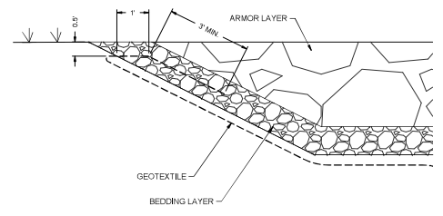
C2 GEOTEXTILE AT CREST DETAIL 22x34: 1" = 1' 11x17: 1" = 2'
