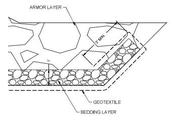
C6 GEOTEXTILE AT TOE DETAIL 22x34: 1" = 1' 11x17: 1" = 2'
