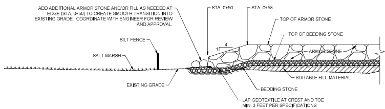
A1 ELEVATION DETAIL AT START OF REVETMENT (STA. 0+50) 22x34: 1" = 6' 11x17: 1" = 12'
