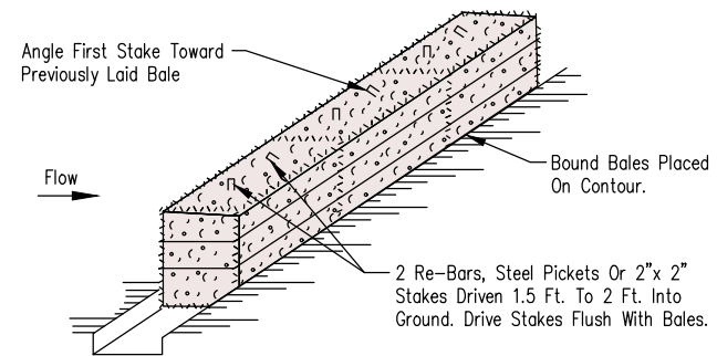
2 TYPICAL HAY/STAW BALE DETAIL Not To Scale
