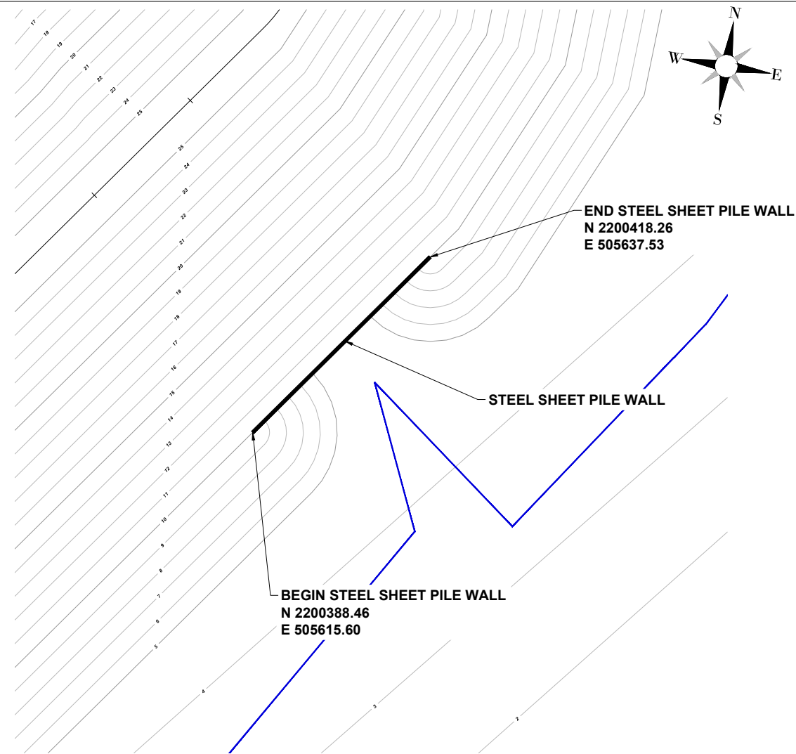
PLAN - STEEL SHEET PILE WALL
