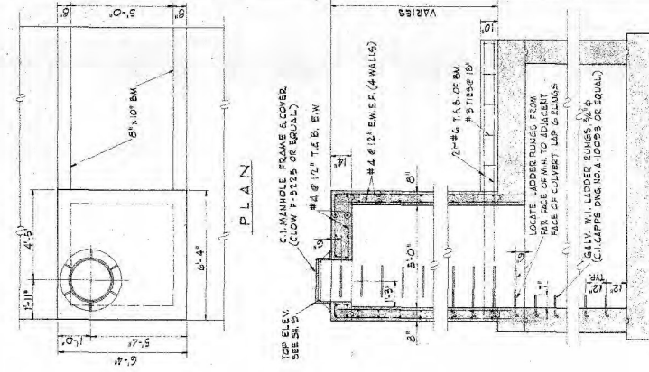
SECTION MANHOLE - DETAIL A SCALE: 3/8" = 1'-0" NOTE: SEE SHEET NO. 9 FOR LOCATIONS (3 READ.)
