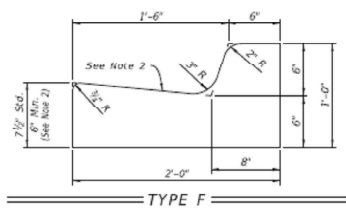
Demo Existing Type F Curb
